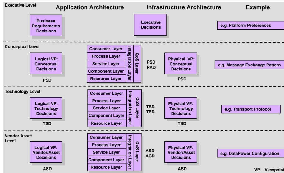
Fig. 11. Layers and levels in RADM for SOA.
